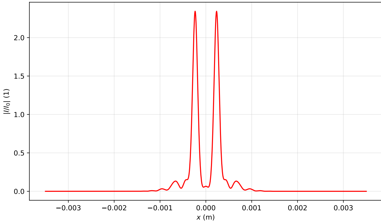
Intensity profile I(x, y = 0, z = 0.716)/I_0 , P_{in}=5.5P_{cr} , artificial time
